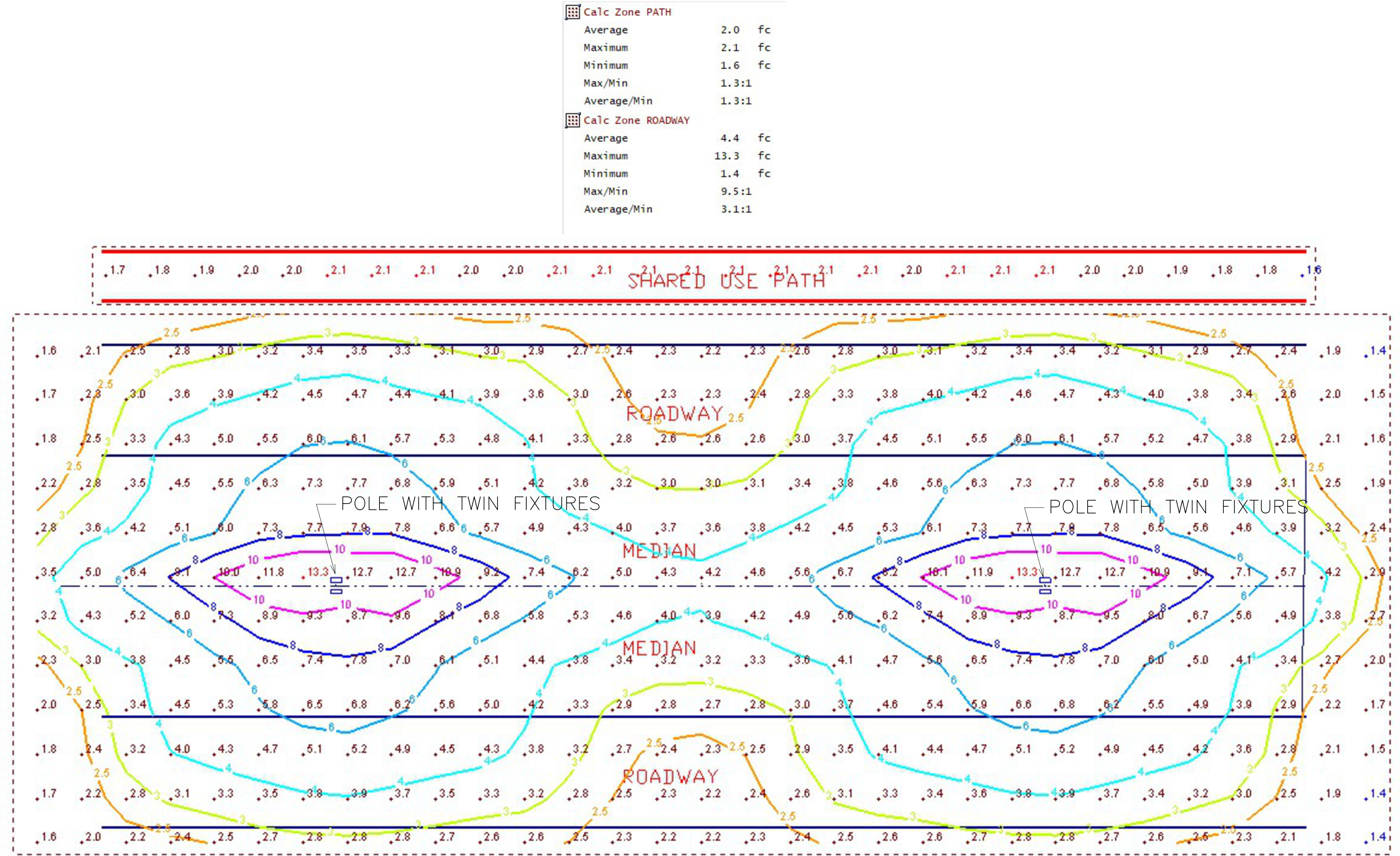
LIGHTING CALCULATIONS (FOOTCANDLES) SCALE: NONE
