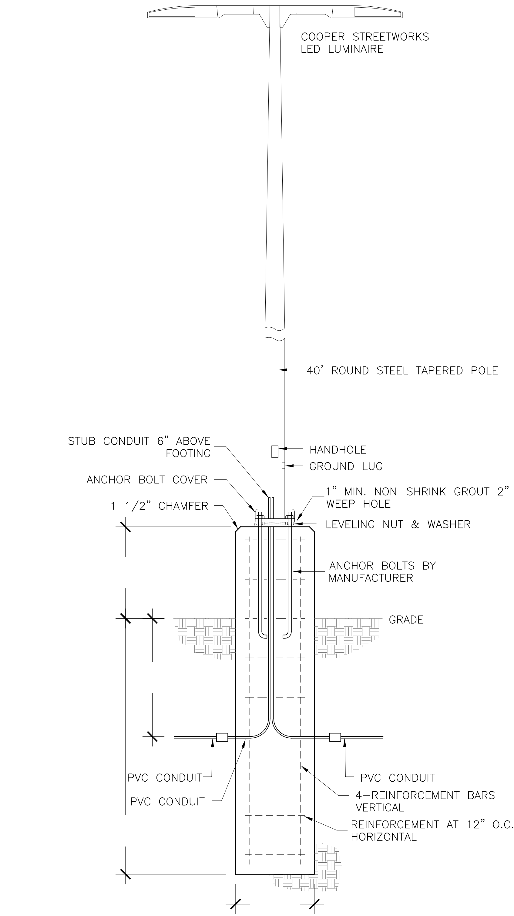
MEDIAN LIGHTING ELEVATION SCALE: NONE
